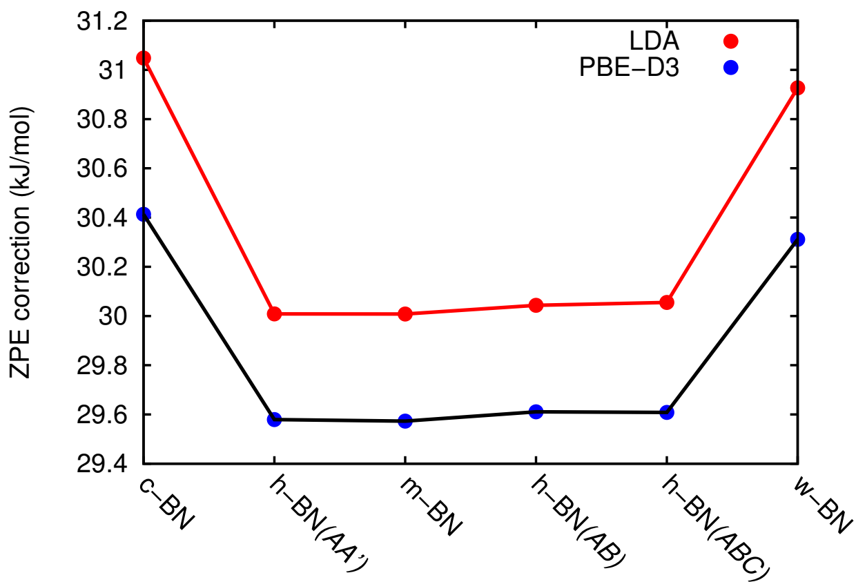
Fig. S5. ZPE corrections accounting for zero-temperature quantum nuclear effects [27] in several BN polymorphs as calculated with the LDA [9] and PBE-D3 [13,14] methods at zero pressure. The ZPE differences estimated among BN polymorphs are practically independent of the employed method.
