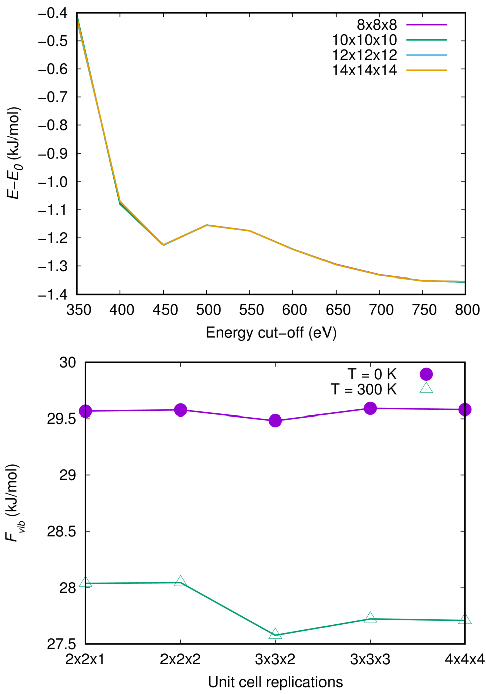
Fig. S4. Convergence tests of the electronic and vibrational free energies calculated with standard DFT methods (i.e., PBE-D3) in the h-BN(AA') polymorph. Electronic energies are converged to within 0.1 kJ/mol (1 meV per formula unit) by using an energy cut-off of 650 eV and 14 \times 14 \times 14 k-point grids. Vibrational free energies are converged to within 0.1 kJ/mol (1 meV per formula unit) by considering 4 \times 4 \times 4 simulation supercells.
