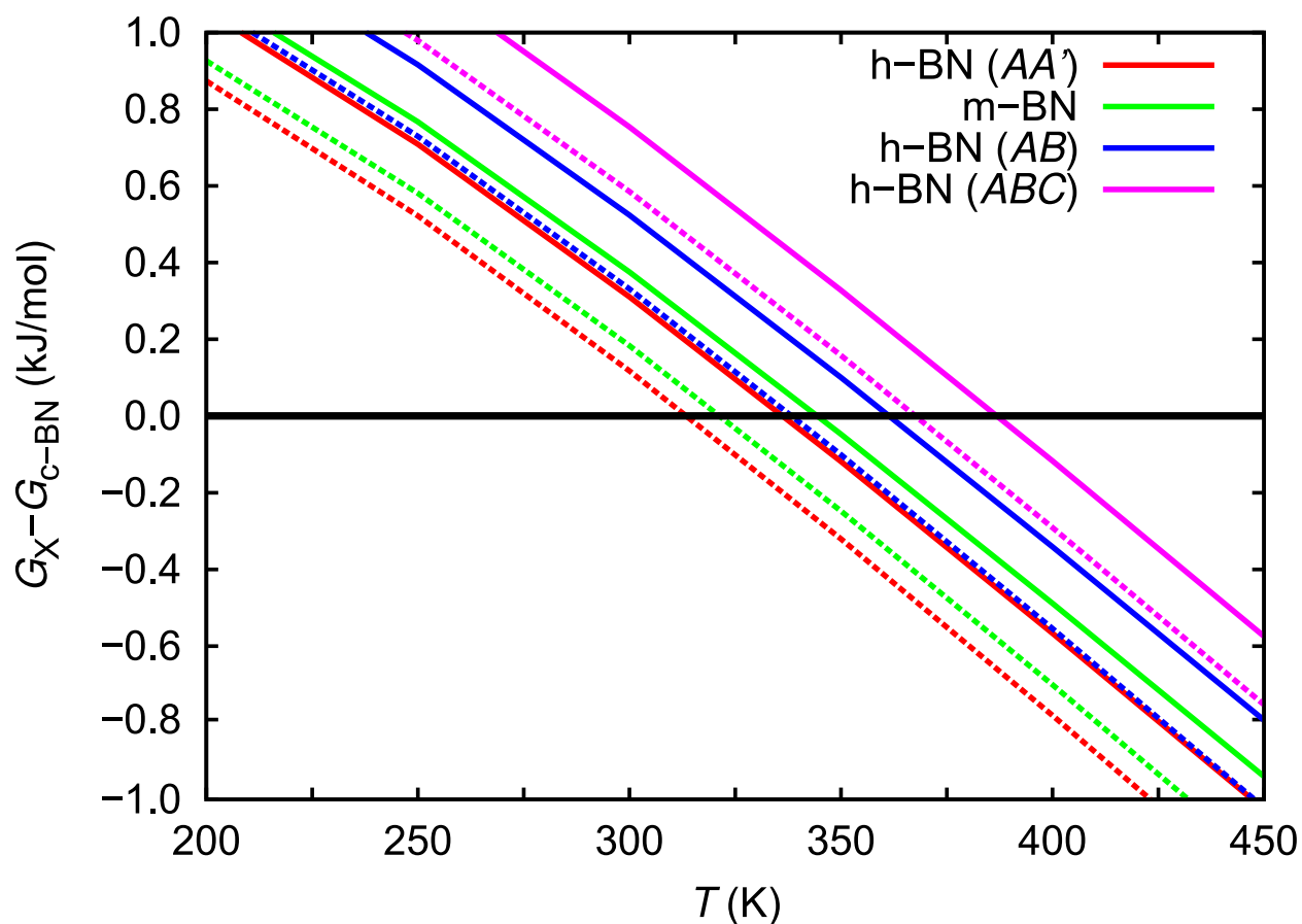
Fig. S2. Gibbs free energy differences among several BN polymorphs calculated at zero pressure and expressed as a function of temperature. Solid lines represent results obtained by considering temperature-induced volume expansion effects, whereas dashed lines represent results obtained by neglecting such effects. When temperature-induced volume expansion effects are disregarded (dashed lines), the transition temperature for the c\text{-BN} \leftrightarrow h\text{-BN}(AA') transformation is underestimated by approximately 25 K.
